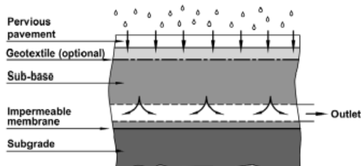
Figure 9(c) - Pervious Pavement System Types: Type C – No Infiltration
