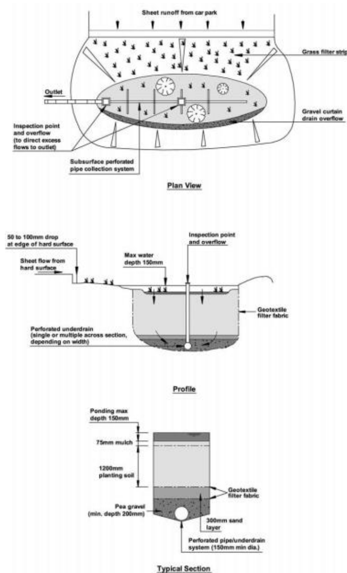
Figure 7 - A Typical Bioretention Configuration
